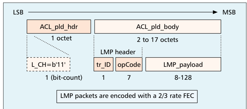
■ Figure 6. The LMP packet format.
