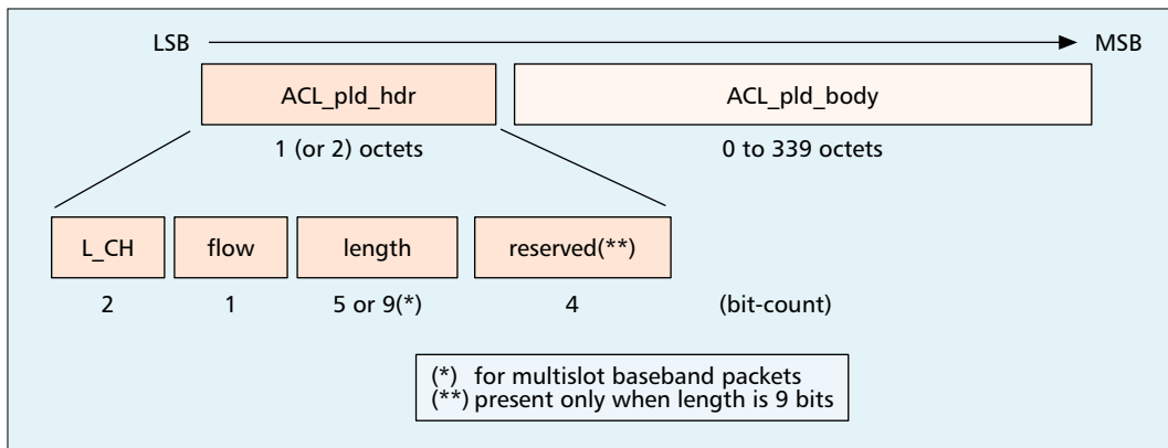
■ Figure 5. The ACL packet payload format.
