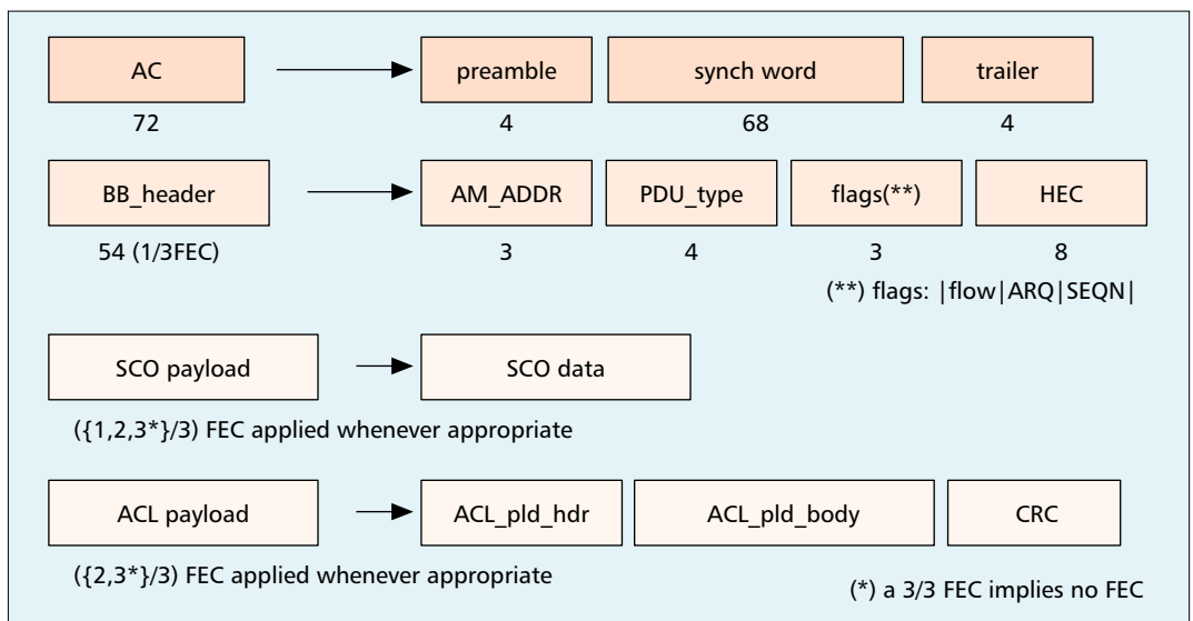
■ Figure 4. The baseband packet fields.
