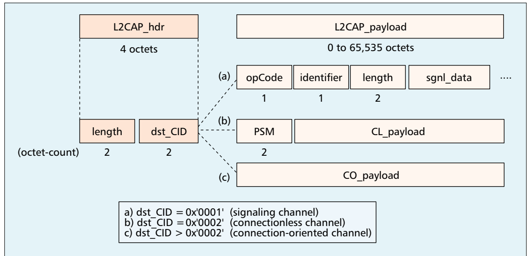
■ Figure 7. The L2CAP packet format.
